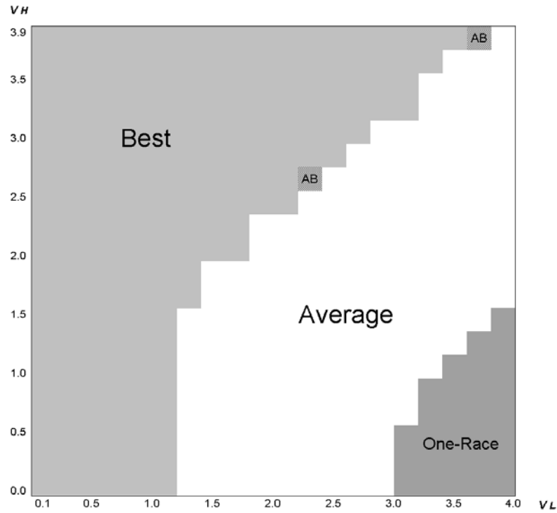
(b) \mu = 2.0
