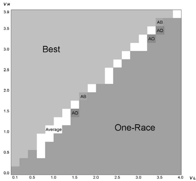
(a) \mu = 0.2
