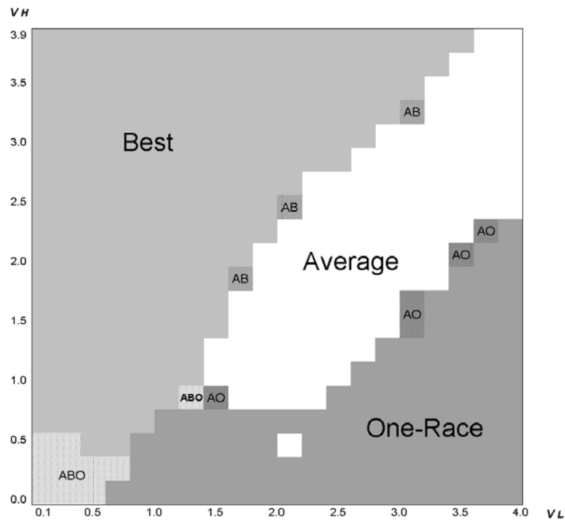
(b) \mu = 2.0
